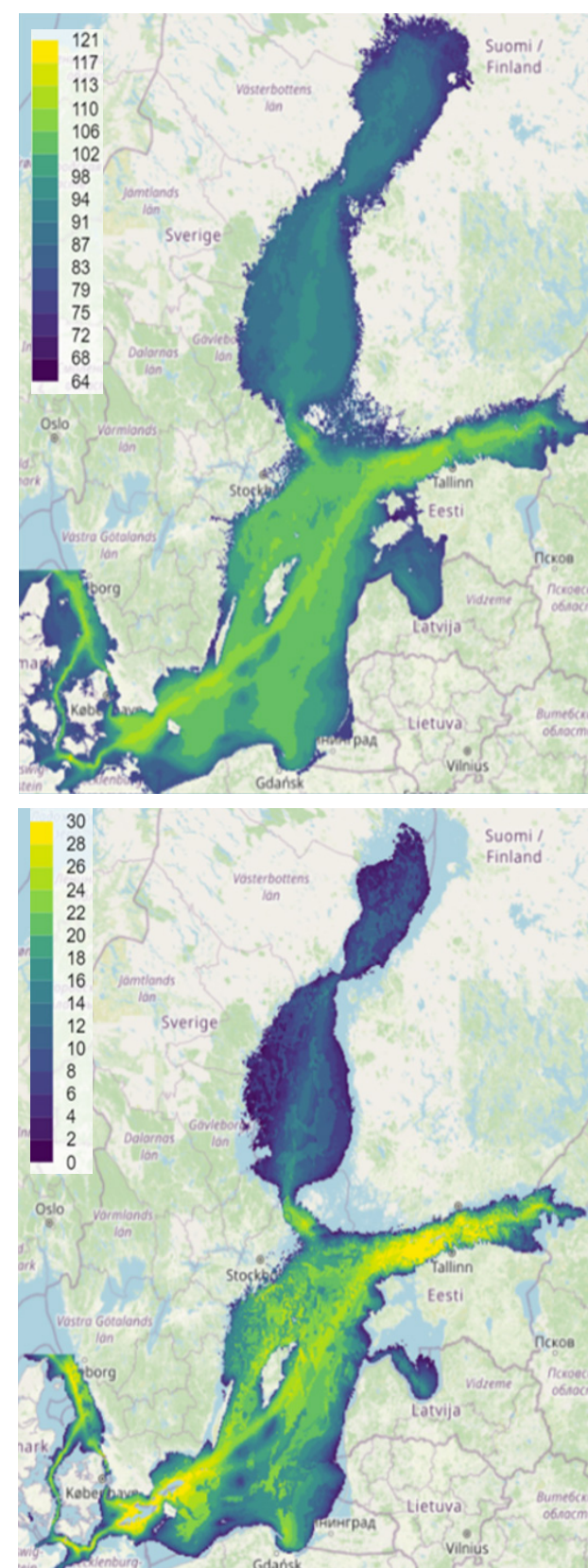
Figure 4.16. Illustration of continuous underwater noise in the Baltic Sea. The upper map shows the median sound pressure level for the third octave band 125 Hz in March 2028, and the map below shows the median excess level for the same. The maps represent the time of the year with the most favourable conditions for the transmission of anthropogenic noise in the Baltic Sea. Source: HELCOM 2023c.
